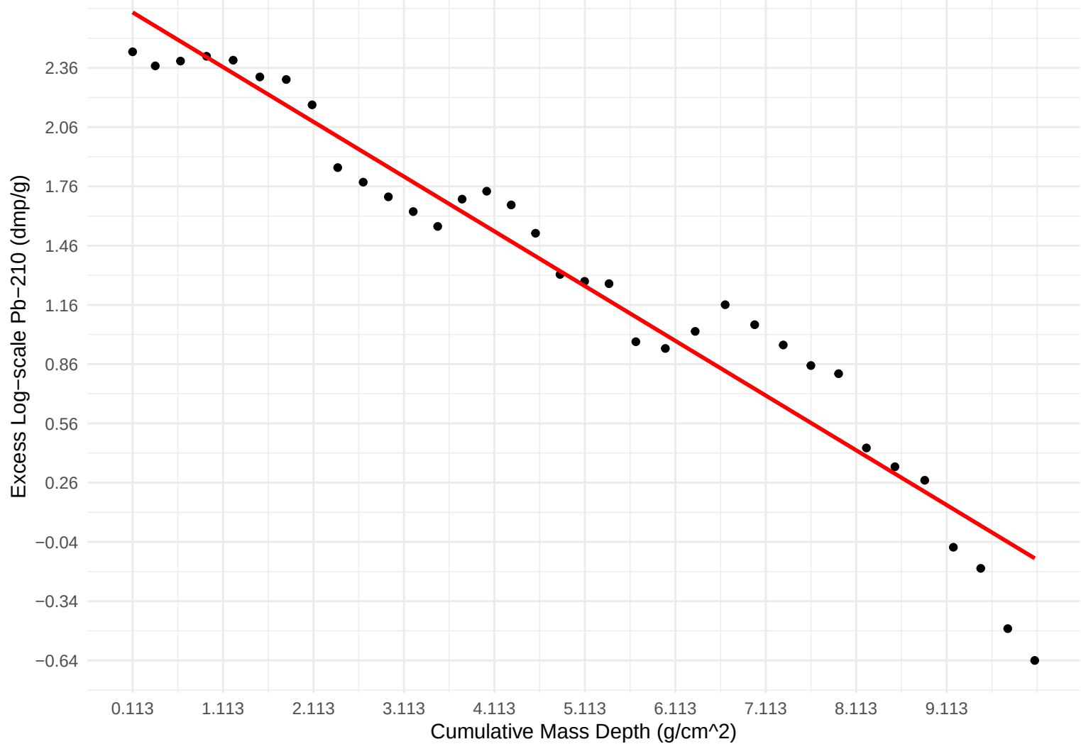
Excess Log-scale Pb-210 vs Mass Depth
